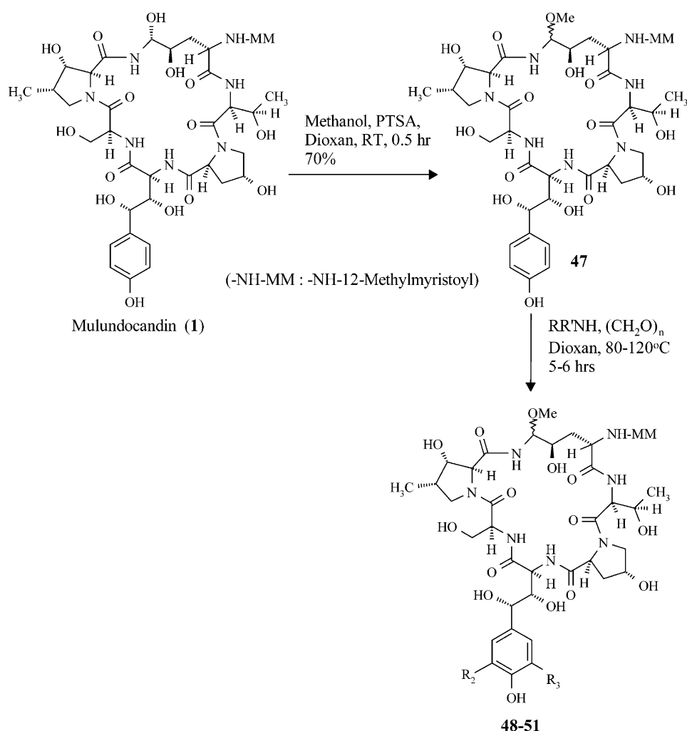
Scheme 5. Mannich reaction on Orn-5-methoxy Mulindocandin ( 47 ).
