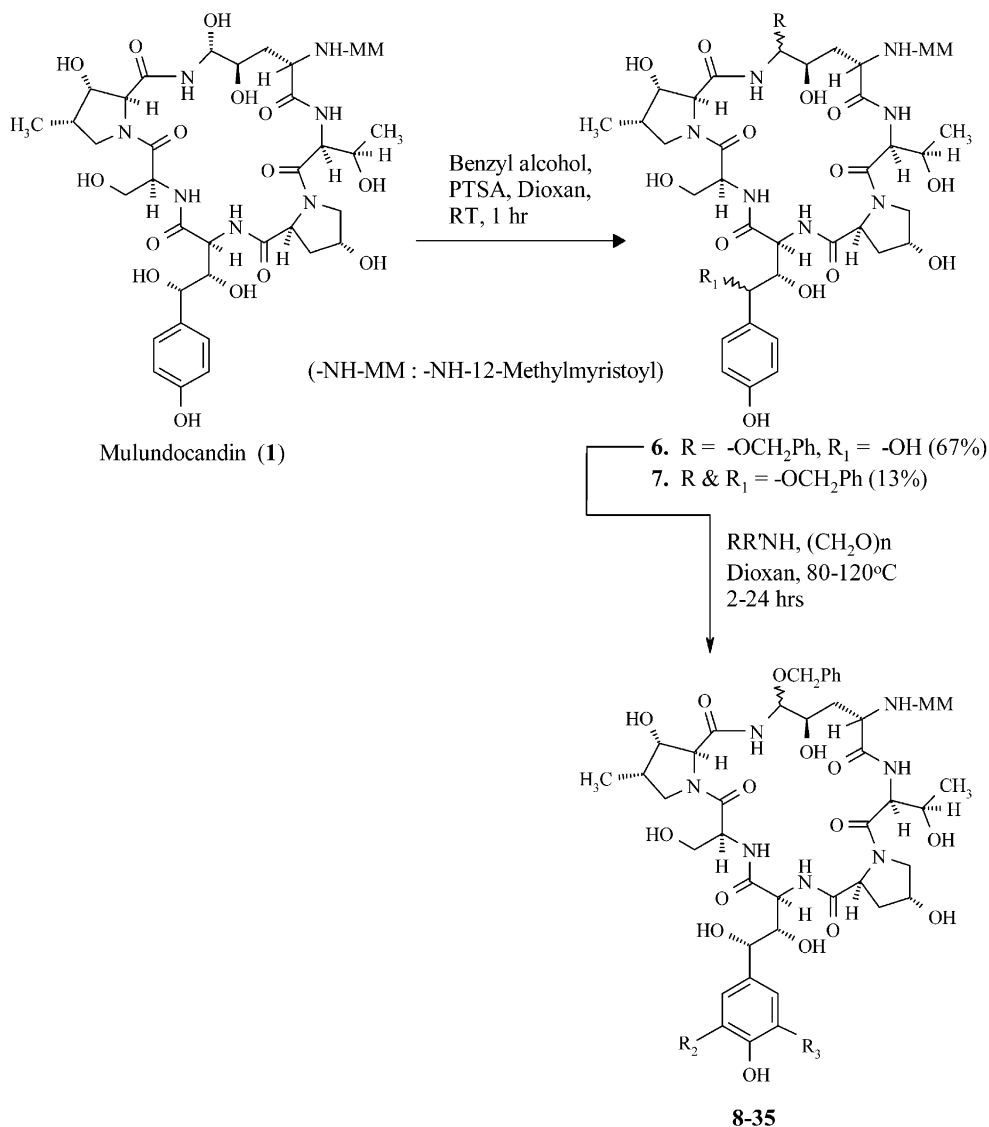
Scheme 2. Mannich reaction on Orn-5-benzyloxy Mulundocandin ( 6 ).
