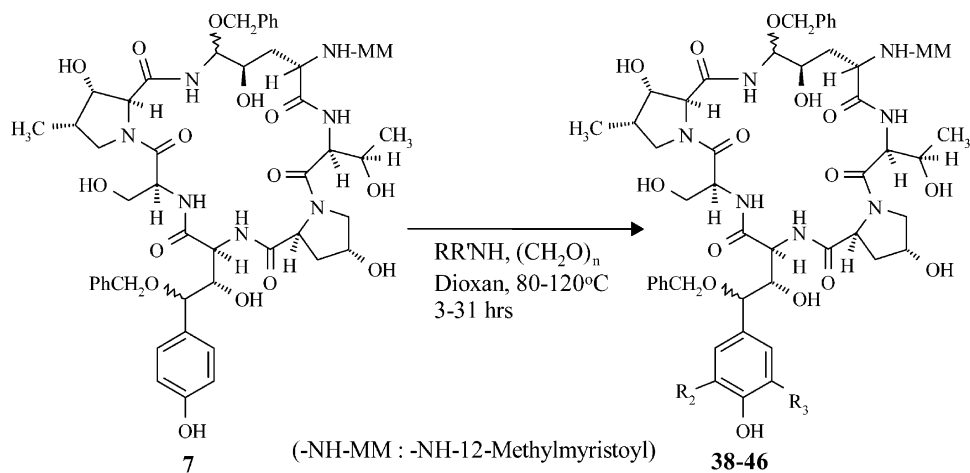
Scheme 4. Mannich reaction on Orn-5- and HTyr-4-dibenzyloxy Mulundocandin ( 7 ).
