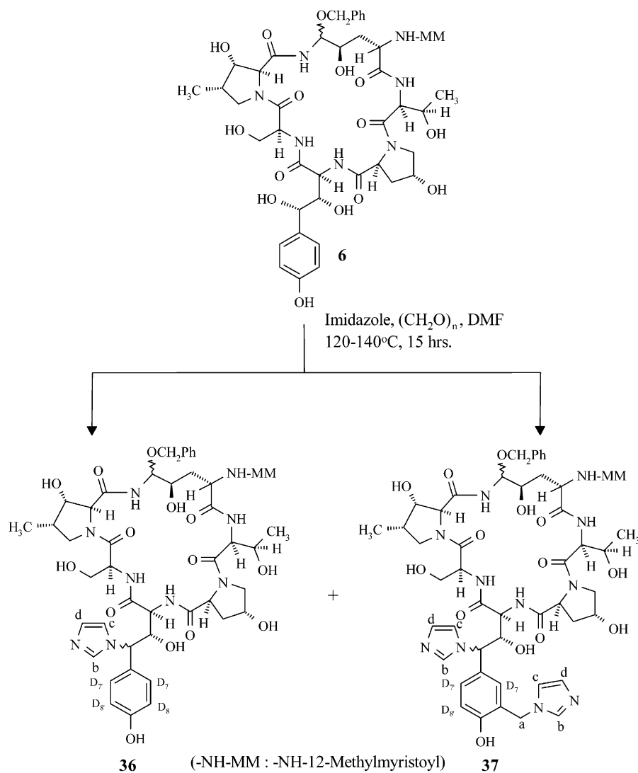
Scheme 3. Mannich reaction on 6 using imidazole as secondary amine.
