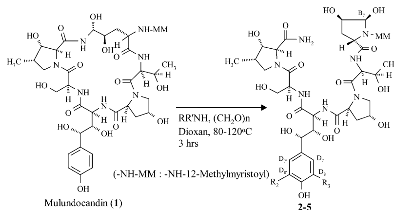
Scheme 1. Mannich reaction on Mulundocandin ( 1 ).
